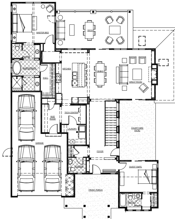
MAIN LEVEL 2064 sq ft
