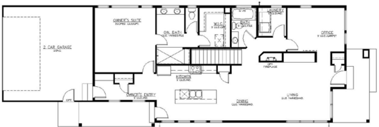
MAIN LEVEL 1328 finished sq ft
