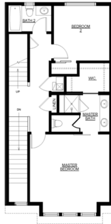
UPPER LEVEL 755 finished sq ft
