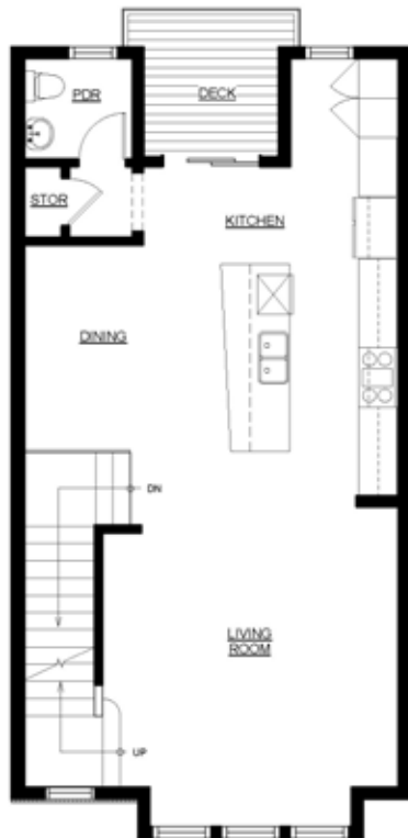
MAIN LEVEL 702 finished sq ft
