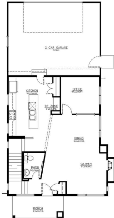
MAIN LEVEL 877 sq ft
