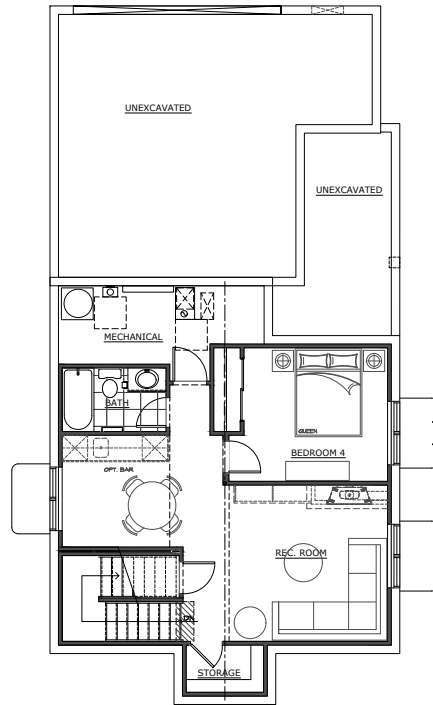
OPTIONAL BASEMENT FINISH 623 sq ft
