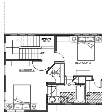
UPPER LEVEL 473 sq ft
